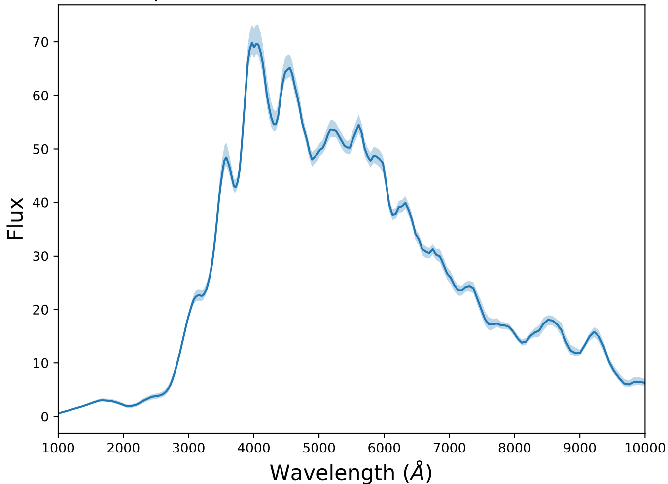
Spectrum 8 for transient SNIa at z=0.84
